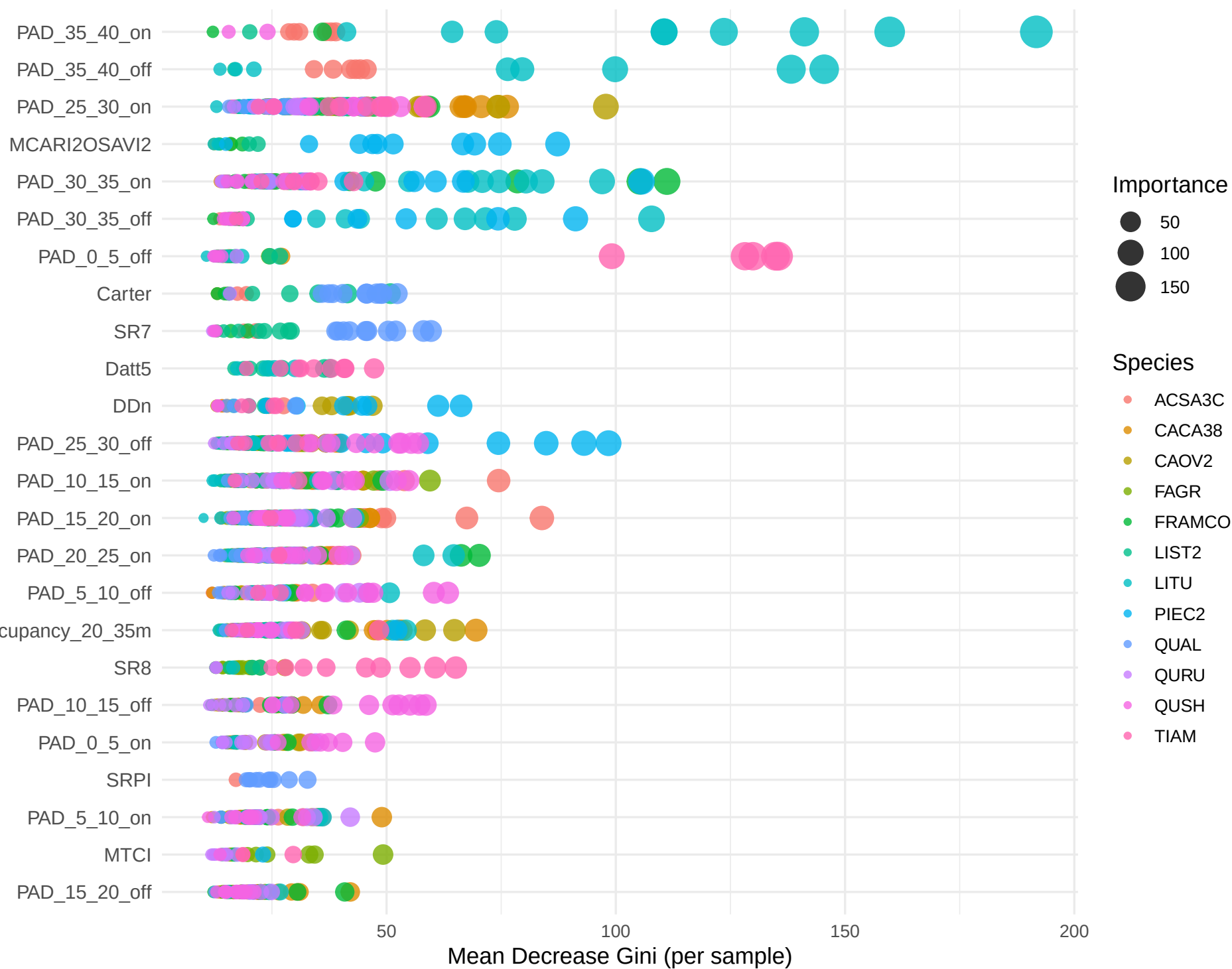
Top 24 Features by Species Mean Importance
